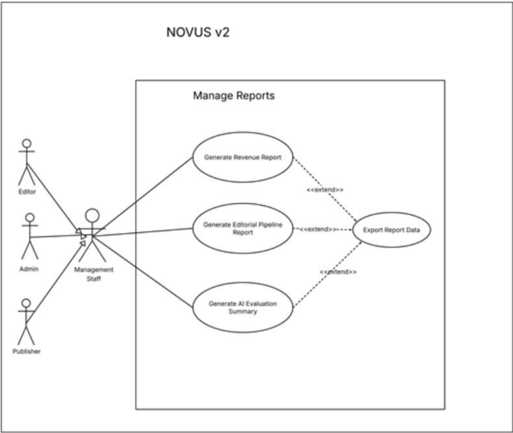
Figure 4. Manage Reports Use Case Diagram
