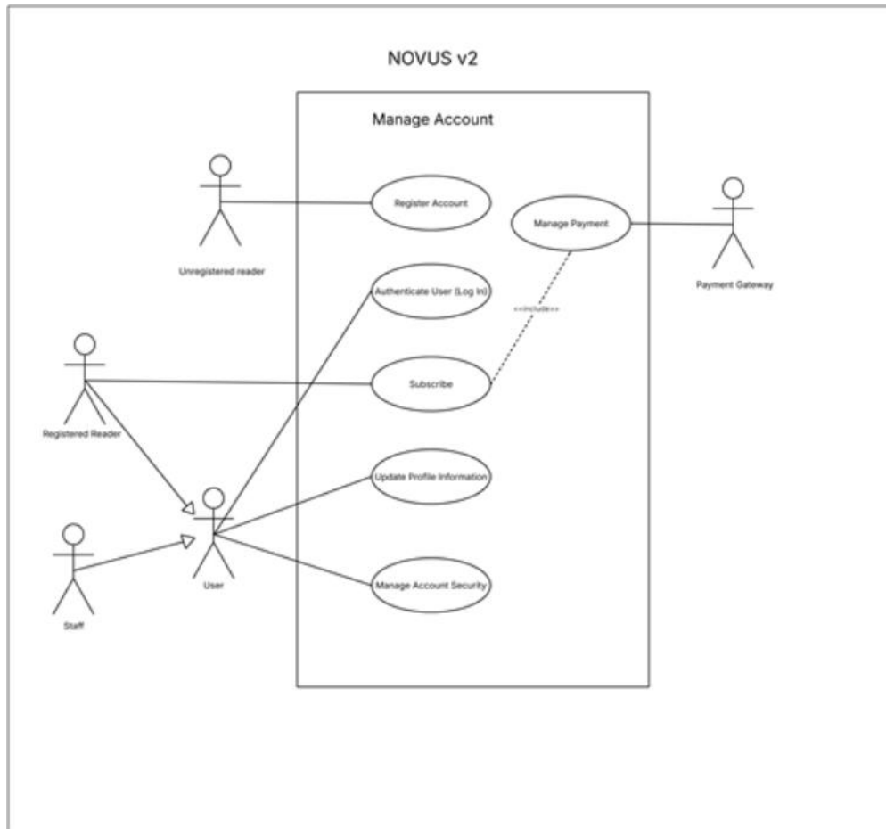
Figure 7. Manage Account Use Case Diagram
