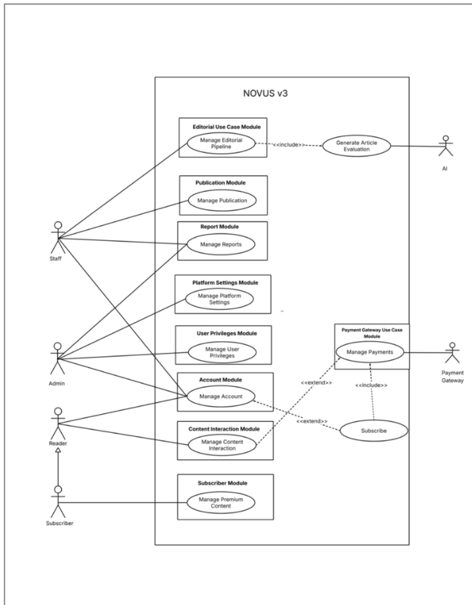
Figure 1. NOVUS Use Case Diagram
