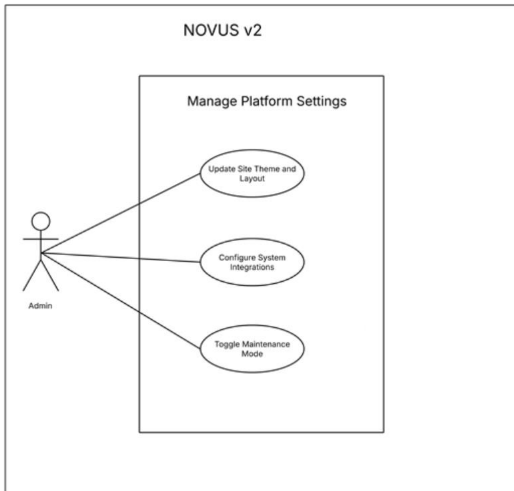
Figure 5. Manage Platform Settings Use Case Diagram
